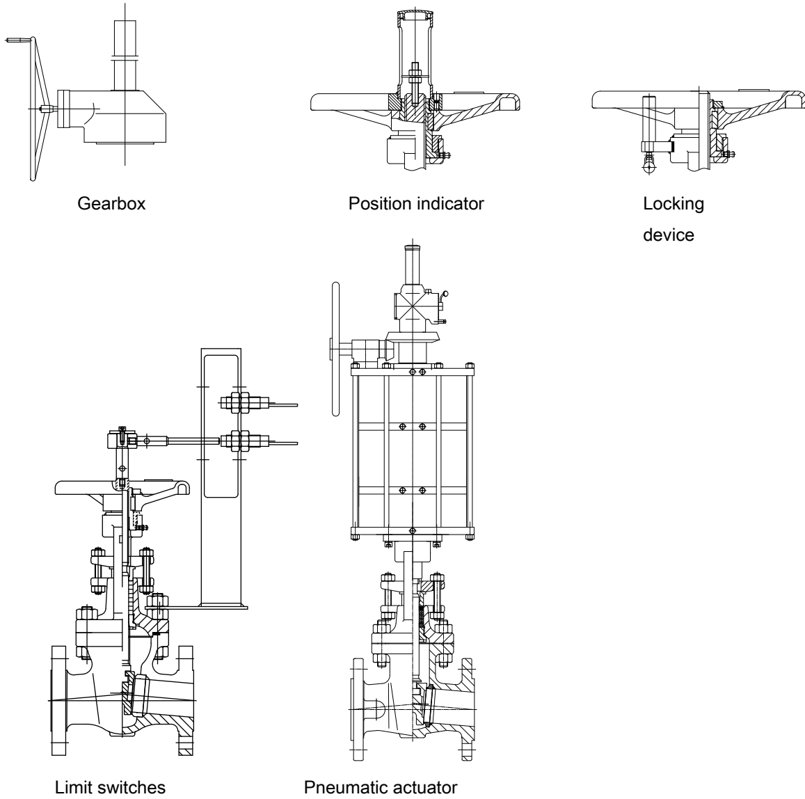
Fig. 2: Sectional drawings
