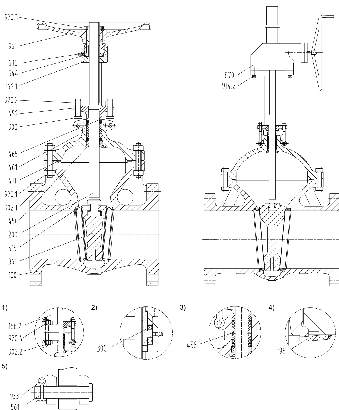
Fig. 1: Sectional drawing 1) Yoke (14 to 24-inch valves, Class 150, 14 to 24-inch valves, Class 300) 2) Bearing (6 to 24-inch valves, Class 600) 3) Lantern ring (optional) 4) Locking plate 5) Split pin
