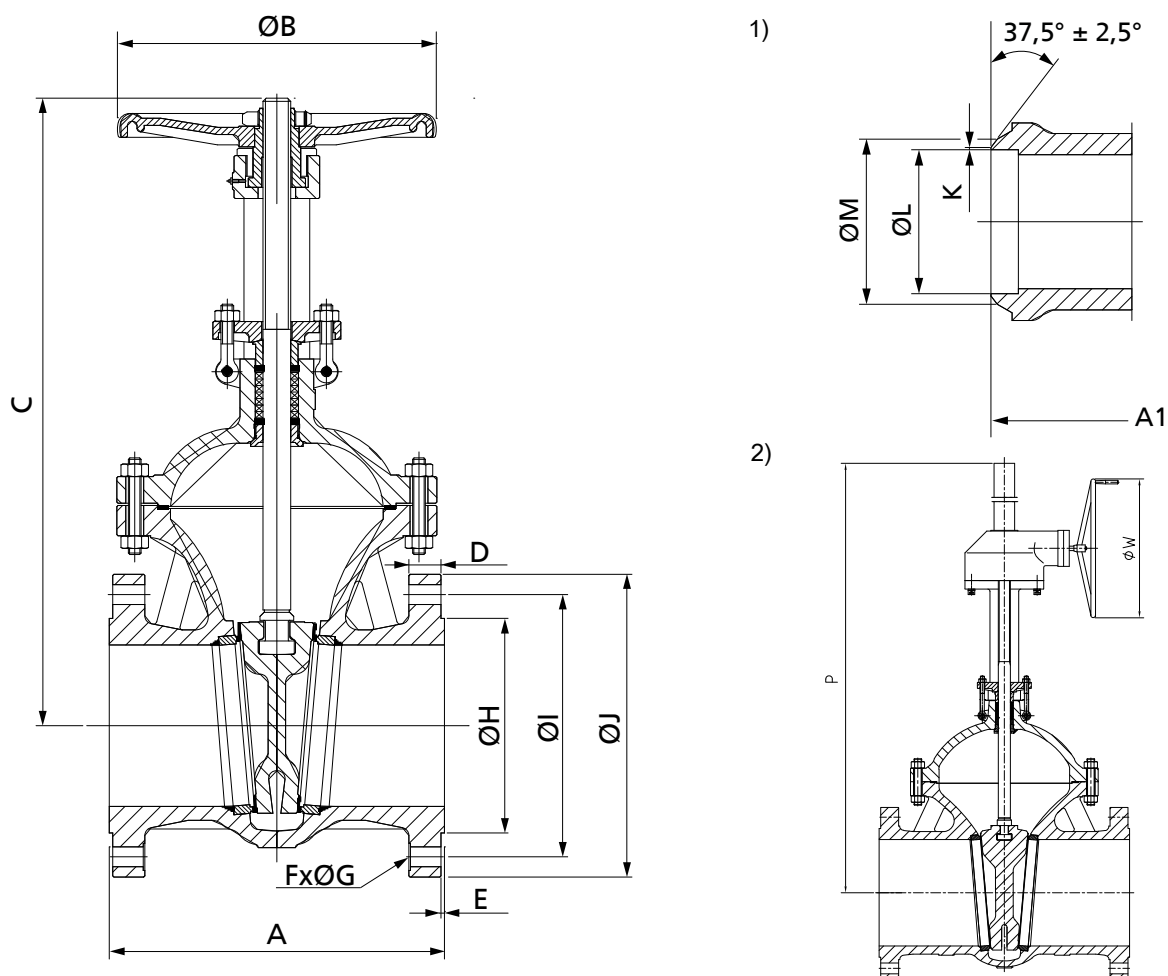
Fig. 3: Dimensions; 1) Butt weld ends; 2) Actuator
