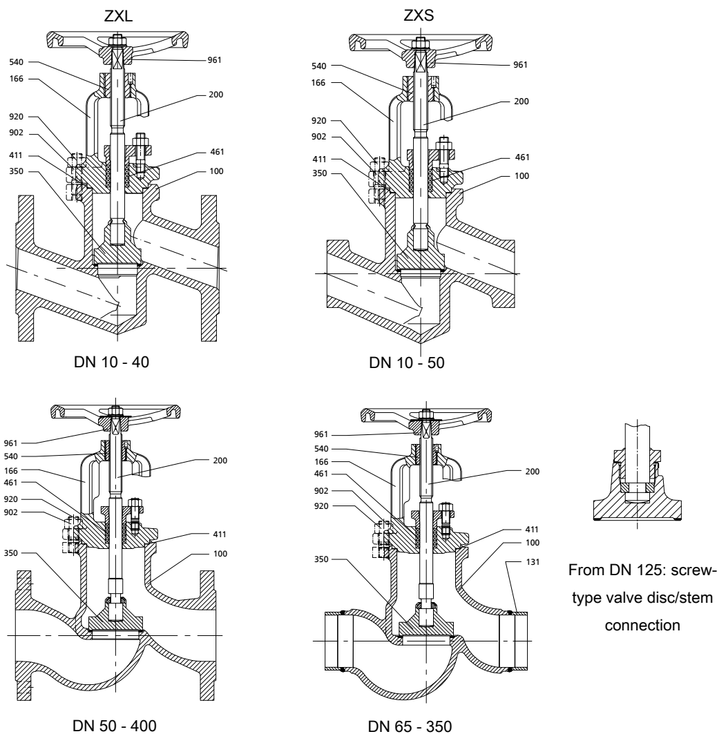
Fig. 1: Sectional drawings
